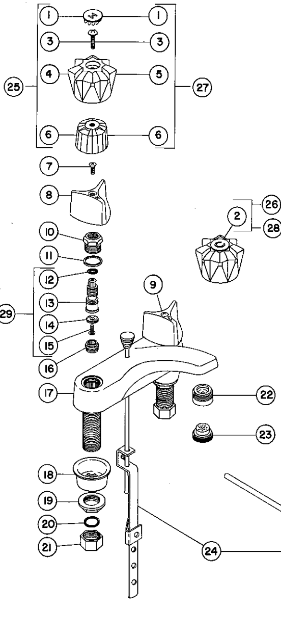
R8020A WITH AERATOR R8020 WITH STREAM GUIDE
