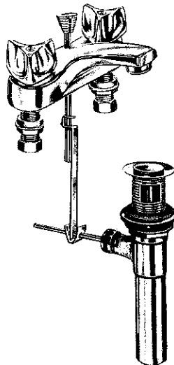
R8020A WITH AERATOR R8020 WITH STREAM GUIDE
